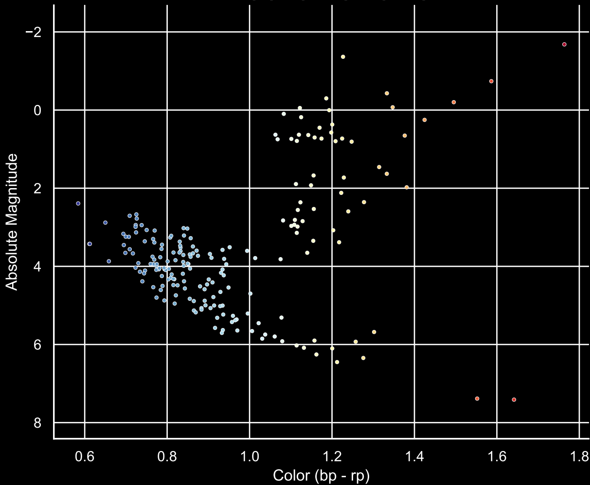
GALAH Hertzprung-Russel Diagram Field [64] Ra [356.52] Dec [-71.96]
