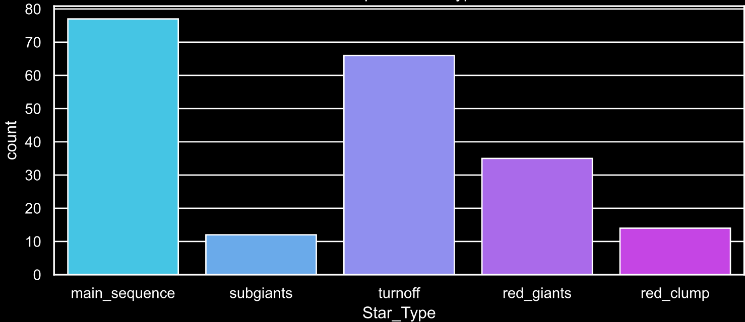
Field [64] Count plot of Star Type
