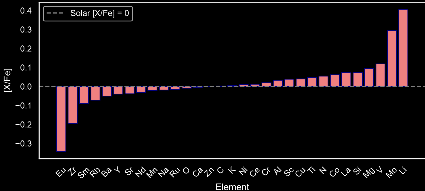
Abundance Pattern for GALAH Main Sequence Stars: Star Field [64] (N=77)
