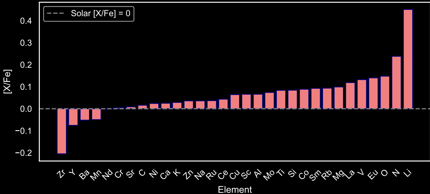
Abundance Pattern for GALAH Star Field [64] (N=204)
