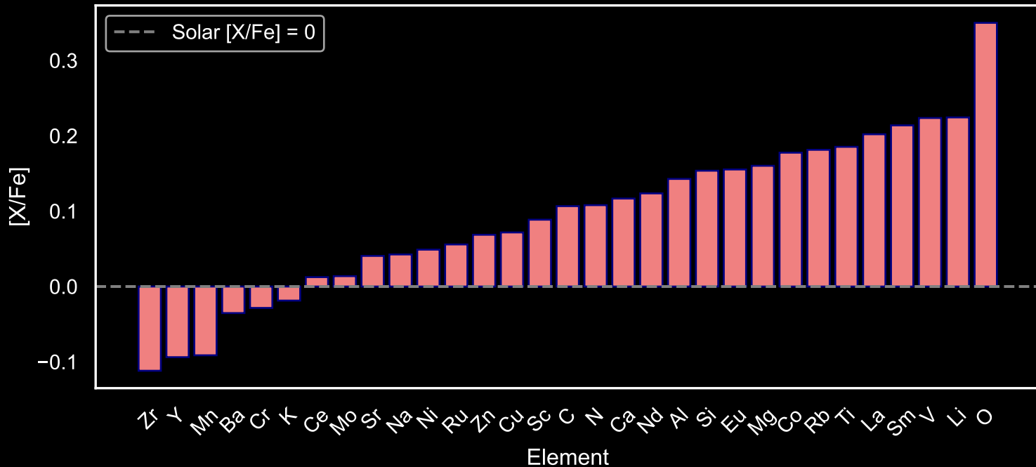
Abundance Pattern for GALAH Red Giants: Star Field [64] (N=49)
